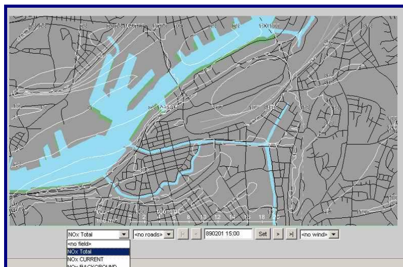
Figure 2.2.2.4. Nesting. Result.
