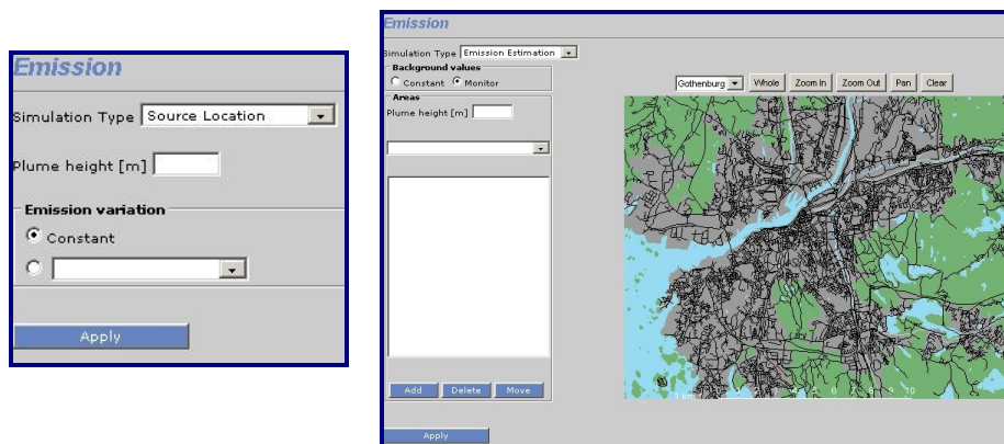
Figure 2.6.3.5. Emission subwindows
