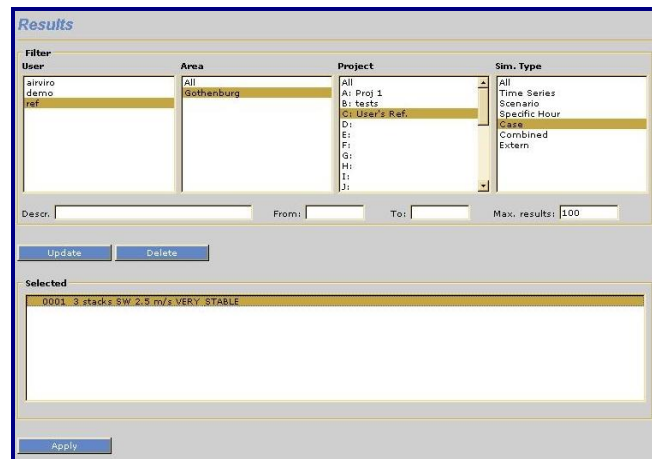
Figure 2.2.2.6. Results.
