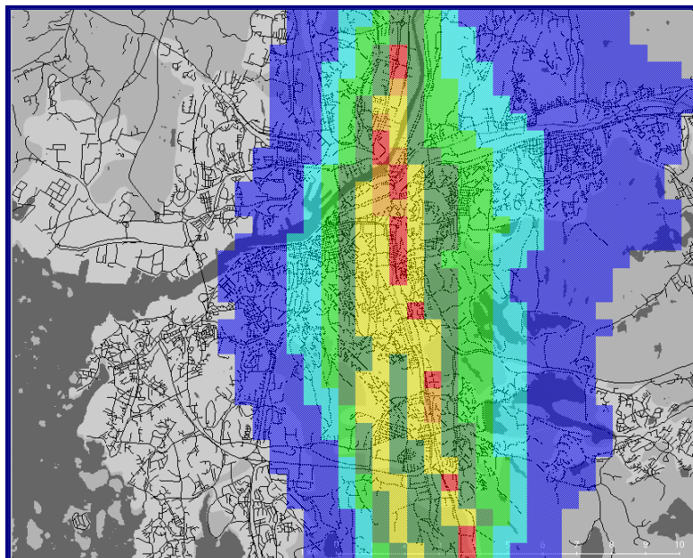
Figure 2.2.2.4 . E6 through Göteborg with winter mean weather conditions, shown as a grid.
