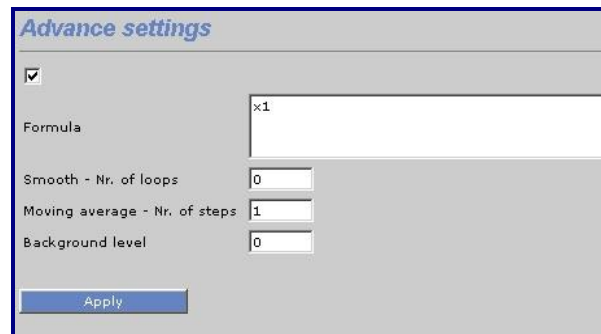
Figure 2.2.5.1. Advance settings.
