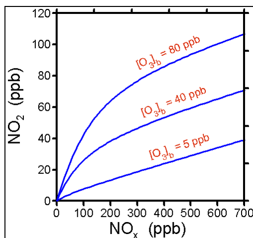
Figure 2J.4. Relation NO 2 -NO x
