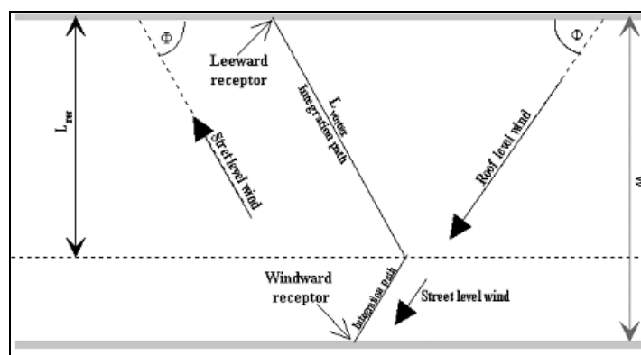
Figure 2J.1. OSPM
