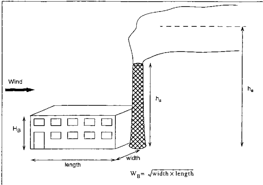
Figure 2C.2 Parameters of interest in the downwash calculation. Find \xi = \min(H_B, W_B) .
