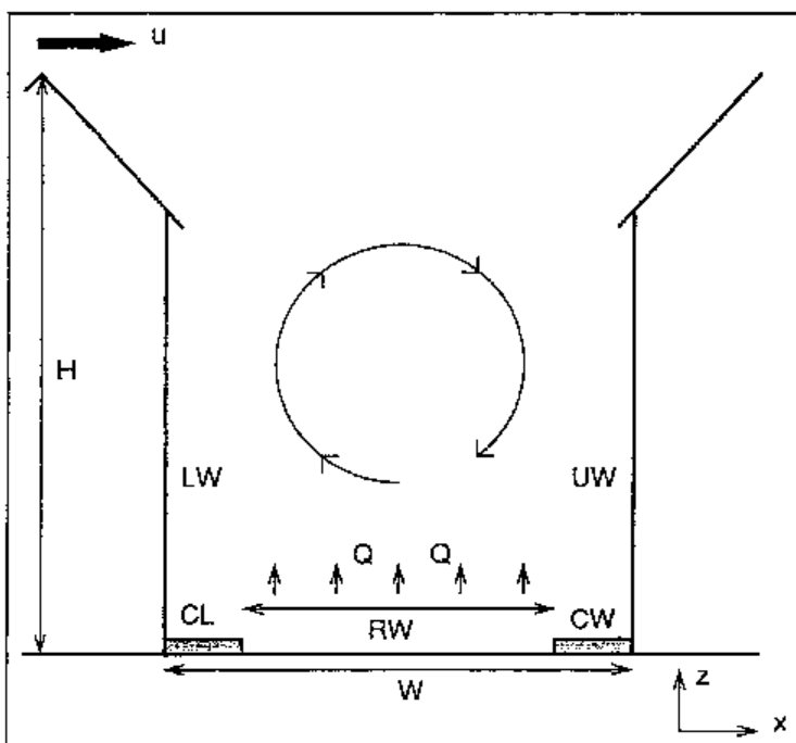
Figure 2E.1 Principles of air circulation within a street canyon (the upwind side is denoted UW , the leewind side LW , see also notations for house height ( H ), street width between houses ( W ) and road width ( RW )).
