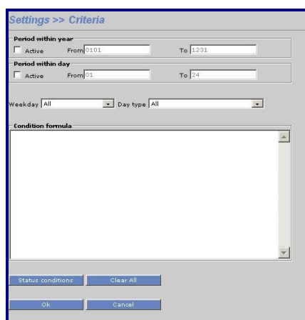
Figure 2.6.3.2. Criteria subwindow
