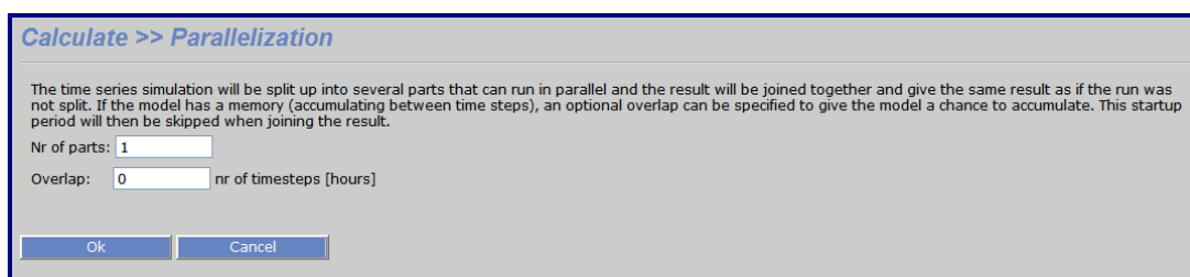
Figure 2.2.2.4 Parallelization
