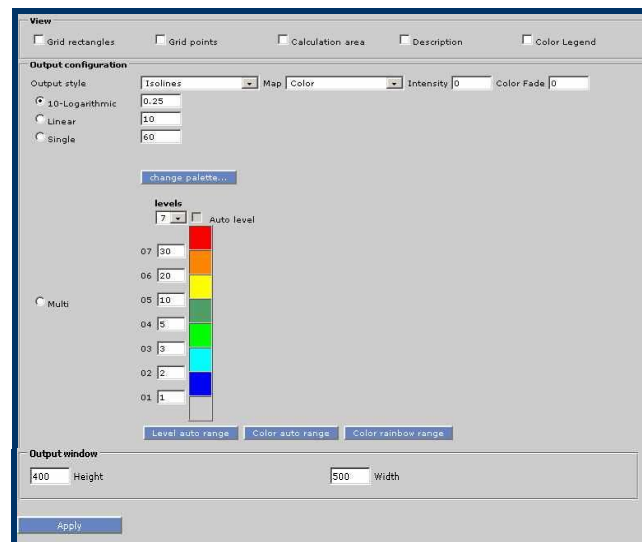
Figure 2.8.3. Output Settings
