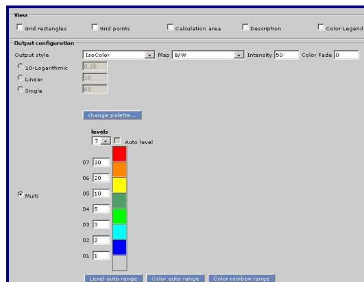
Figure 2.7.4. Output Settings
