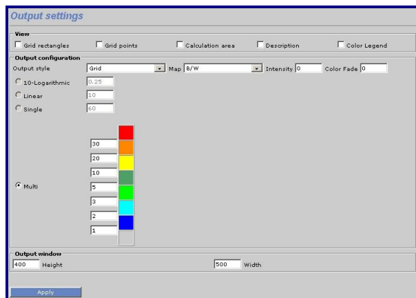
Figure 2.2.2.3. Output settings
