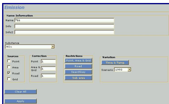
Figure 2.2.2.1. Emission
