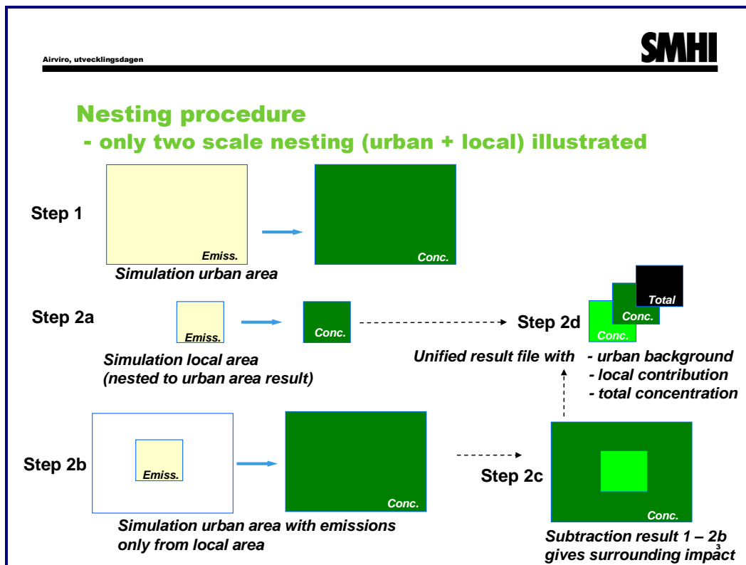
Figure 2.2.2.2. Nesting operation.
