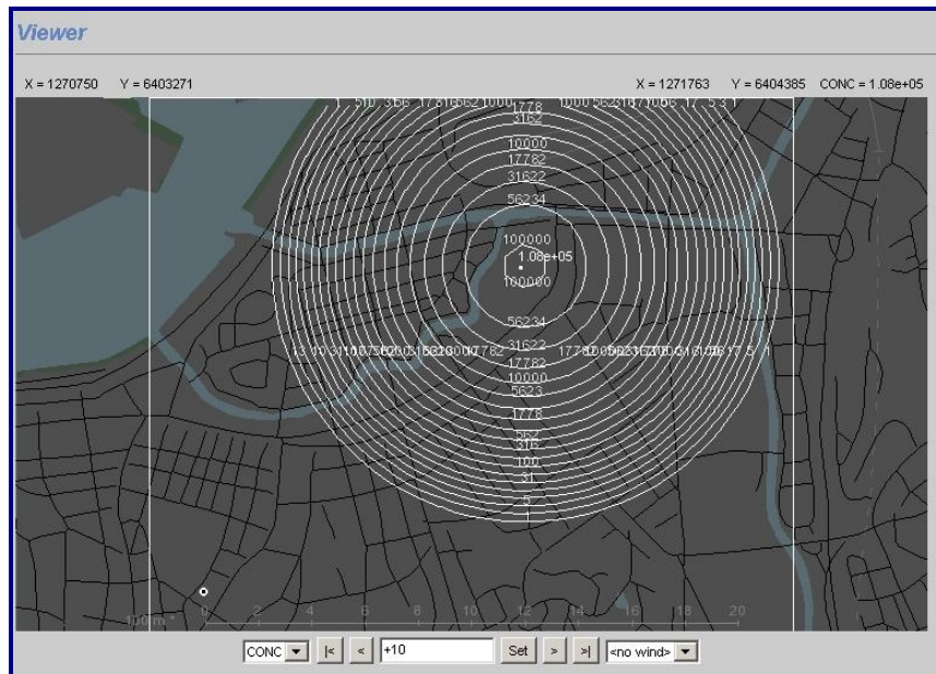
Figure 2.5.3 Ammonia leakage from a tank burst, 10 minutes after the burst.
