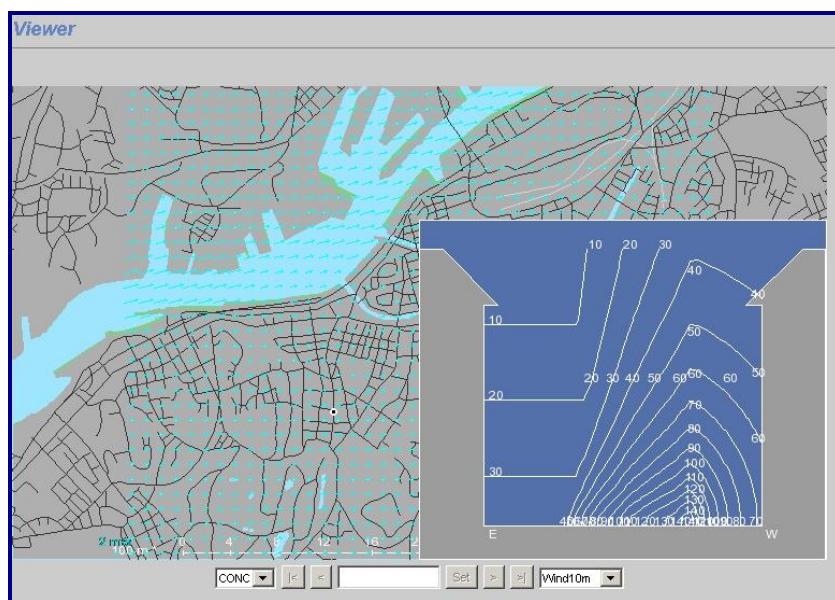
Figure 2.3.1.3. Canyon model of a typical summer west wind across Linnégatan
