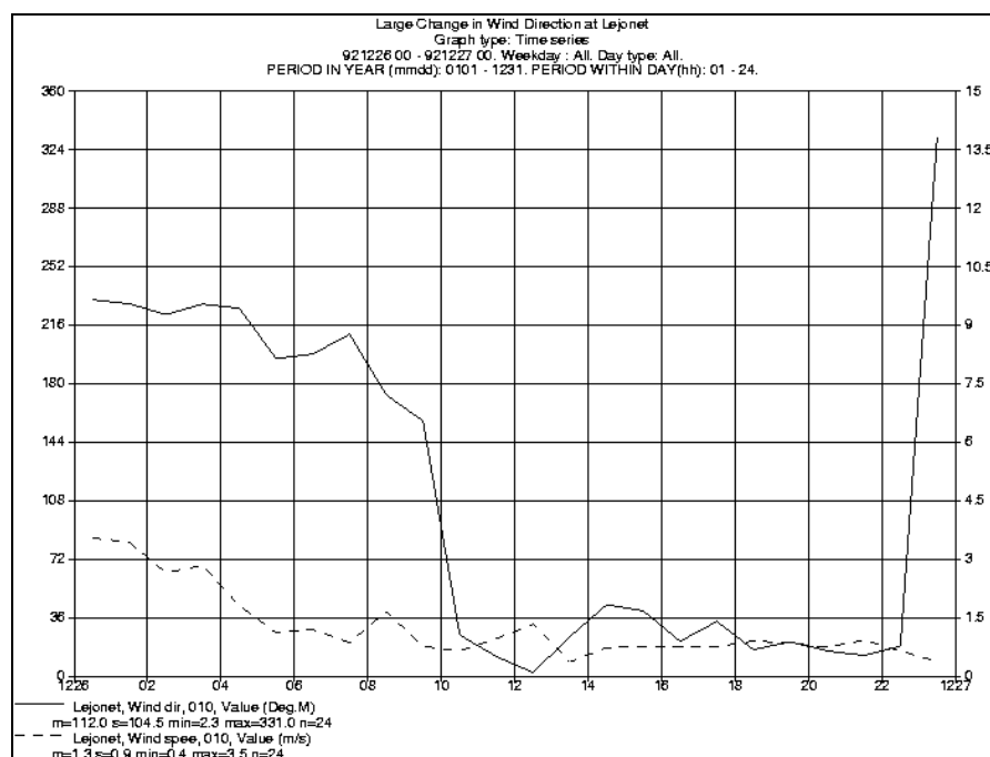
Figure 2.4.1 Wind speed and direction at Lejonet 921226
