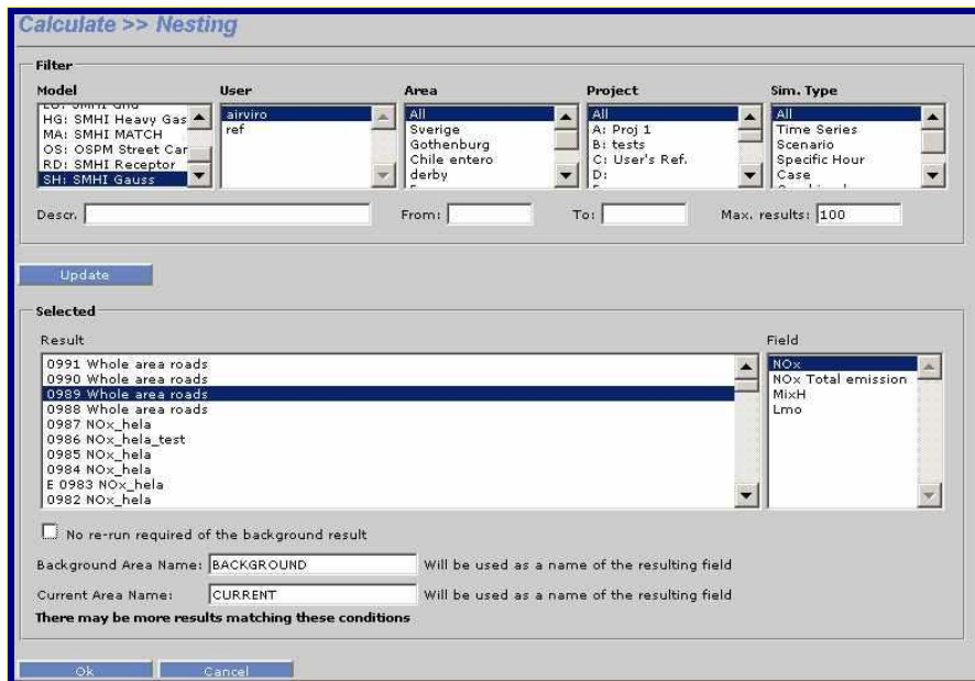
Figure 2.2.2.3. Calculate. Nesting
