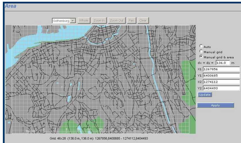
Figure 2.8.2. Area
