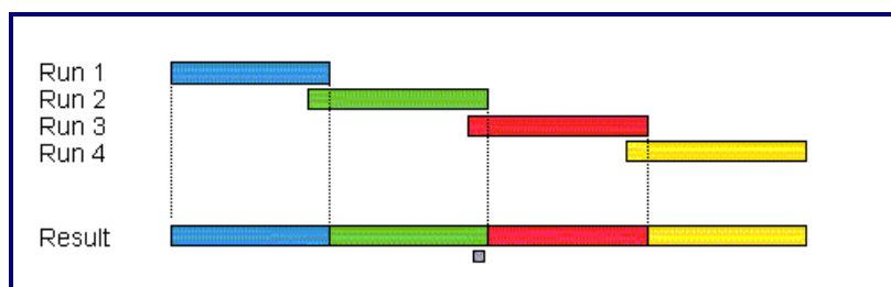
Figure 2.2.2.5 Example Parallelization
