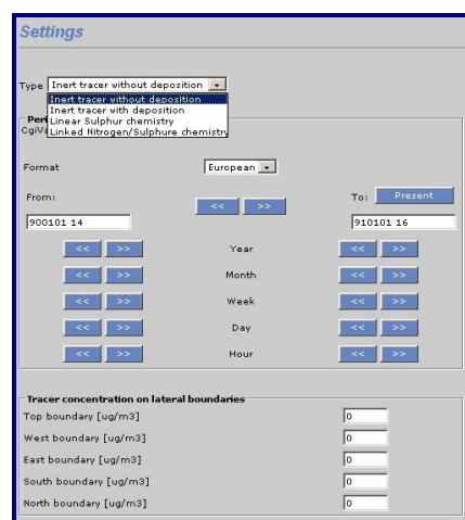
Figure 2.8.1. Settings
