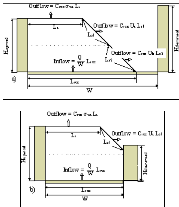
Figure 2J.3. Recirculation
