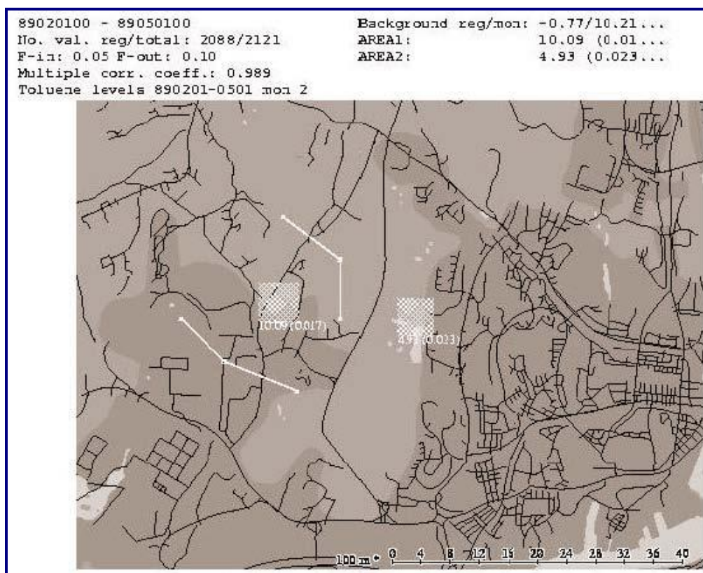
Figure 2.6.5.1. Result
