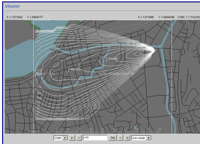
Figure 2.5.2. Simulation of Chlorine levels from 920524 12, 10 minutes after a leak began
