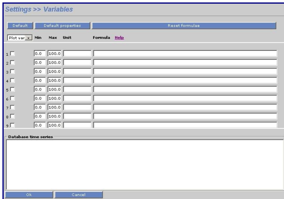
Figure 2.6.3.2. Variables subwindow
