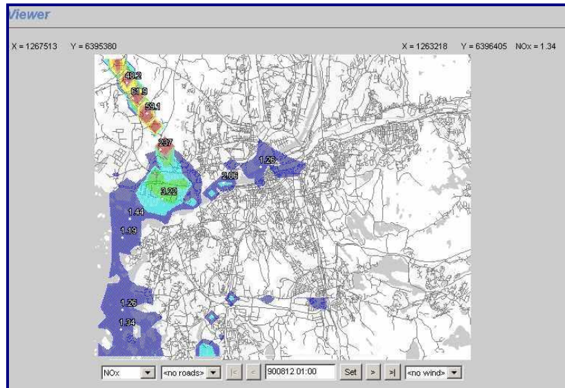
Figure 2.7.3. Viewer
